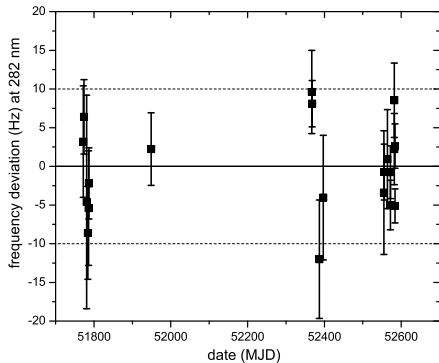
FIG. 3: Absolute frequency measurements of the ^{199}\text{Hg}^+ \ ^2S_{1/2}(F=0) \longleftrightarrow \ ^2D_{5/2}(F=2) transition with respect to the ^{133}\text{Cs} ground state hyperfine splitting defining the SI second. The plot shows the deviation of each measurement from the weighted average value with its statistical \pm 1\sigma error bar. The horizontal axis is the Modified Julian Date (MJD 52582 = Nov. 4, 2002).
