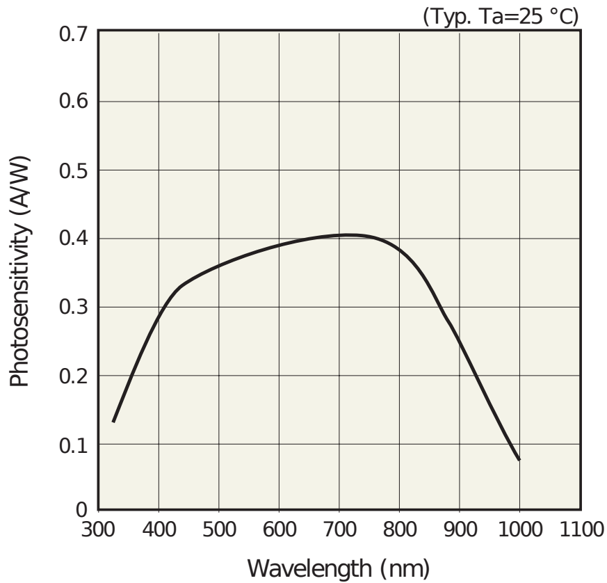
Figure 1: Photosensitivity of the Hamamatsu S5973-02 Si-Photodiode. Source: Hamamatsu Photonics K.K., "Si PIN photodiodes S5971, S5972, S5973 series", S5973-02 datasheet, Nov. 2019, page 2
