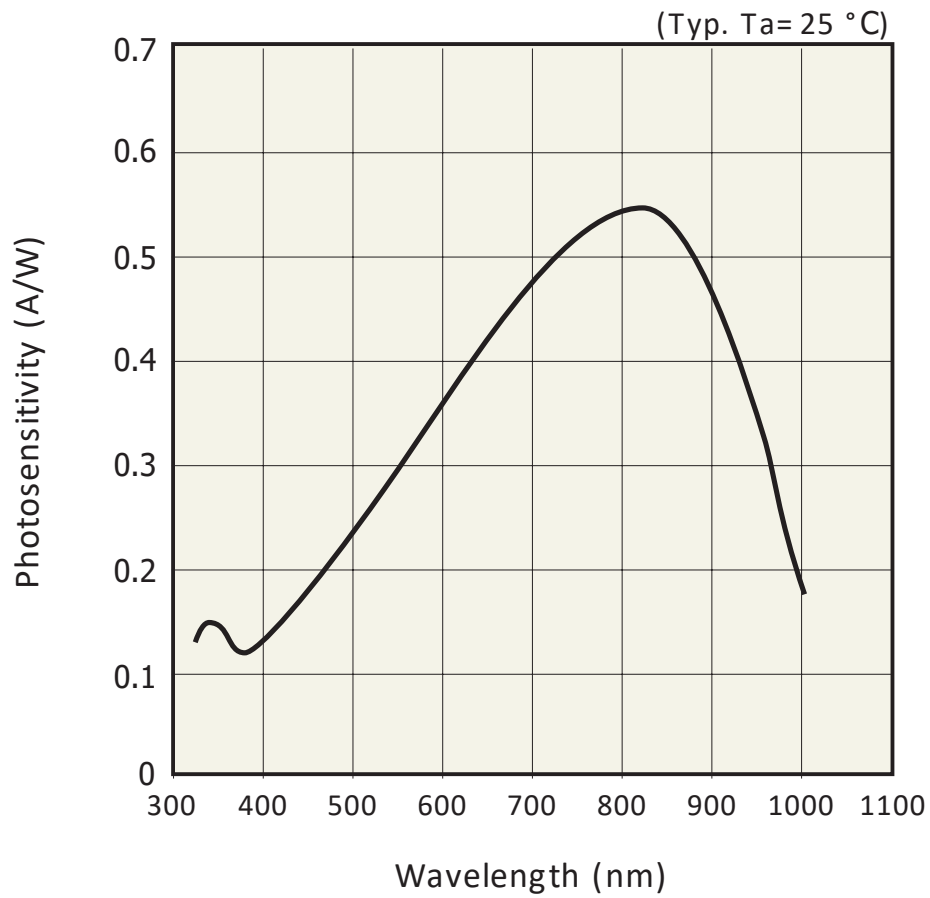
Figure 1: Photosensitivity of the Hamamatsu S5972 Si-Photodiode. Source: Hamamatsu Photonics K.K., "Si PIN photodiodes S5971, S5972, S5973 series", S5972 datasheet, Nov. 2019, page 2
