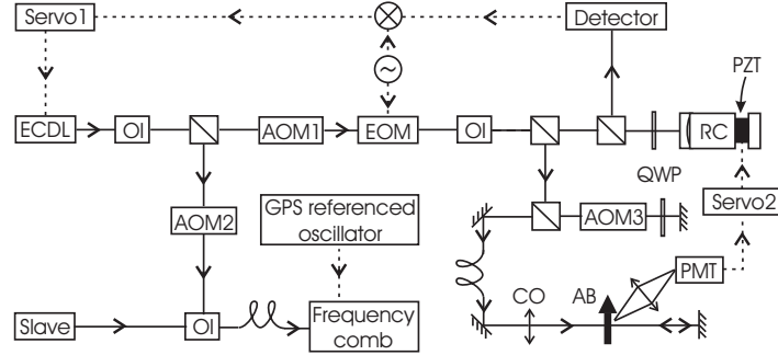
Fig. 18. Scheme of the 689 nm laser. Experimental setup used for the frequency measurement on the Sr intercombination line. Optical isolators (OI) and acousto-optic modulators (AOM) eliminate feedback among the master laser (ECDL), the slave laser, the electro-optic modulator (EOM) and the reference cavity (RC). QWP: quarter wave-plate. CO: collimation optics. PMF: polarization maintaining fiber. PMT: photo multiplier tube. The same apparatus is used for Sr second stage cooling and trapping, but the thermal beam is replaced by a heat-pipe.
