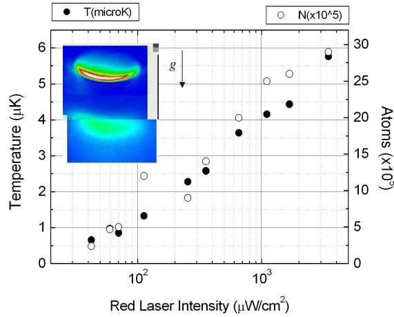
Fig. 4. Measured atomic temperature and population of the red MOT as a function of the laser intensity with our apparatus. The inset shows in-situ and free-fall images of the trapped atoms.
