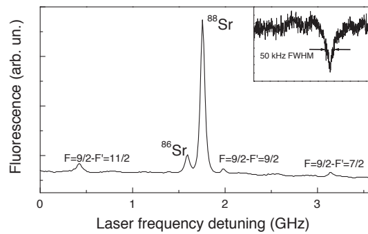
Fig. 14. Fluorescence spectrum of the strontium 1S_0-3P_1 line at 689 nm. The lines of the two bosonic isotopes ^{86}\text{Sr} and ^{88}\text{Sr} , together with the hyperfine structure of the fermionic ^{87}\text{Sr} , can be resolved. The linewidth corresponds to the residual first order Doppler broadening in the thermal beam. Inset: sub-Doppler resonance of ^{88}\text{Sr} recorded by saturation spectroscopy using two counterpropagating laser beams. The amplitude of the dip is 10 % of the Doppler signal. Reprinted figure with permission from G. Ferrari et al., Phys. Rev. Lett. 91, 243002 (2003). Copyright (2006) by the American Physical Society.
