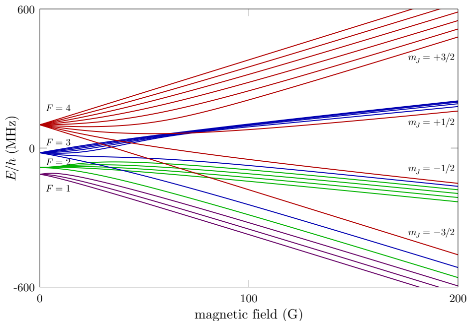
Figure 6: Rubidium 85 5^2P_{3/2} ( D_2 excited) level hyperfine structure in an external magnetic field. The levels are grouped according to the value of F in the low-field (Zeeman) regime and m_j in the strong-field (hyperfine Paschen-Back) regime.
