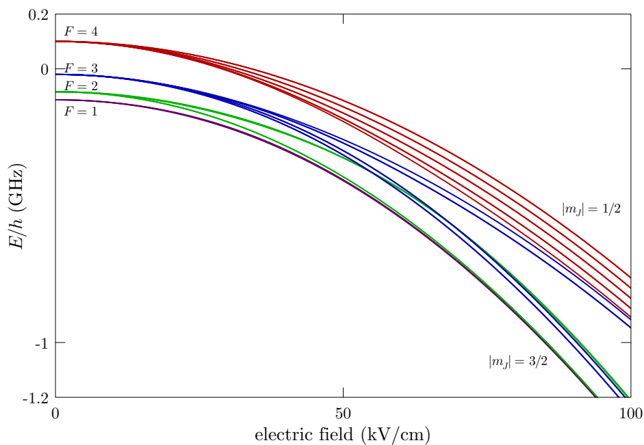
Figure 7: Rubidium 85 5^2P_{3/2} ( D_2 excited) level hyperfine structure in a constant, external electric field. The levels are grouped according to the value of F in the low-field (Zeeman) regime and |m_j| in the strong-field ("electric" hyperfine Paschen-Back) regime. Levels with the same values of F and |m_F| (for a weak field) are degenerate.
